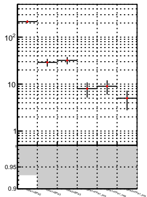
N of reco track vs. \chi^2 oob
