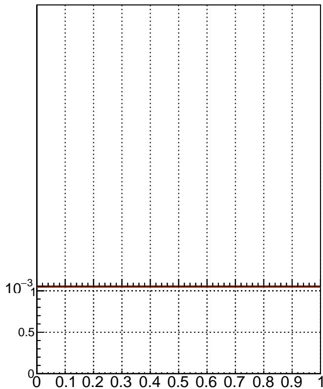
RecoPVAssoc2GenPVNotMatched_Purity
