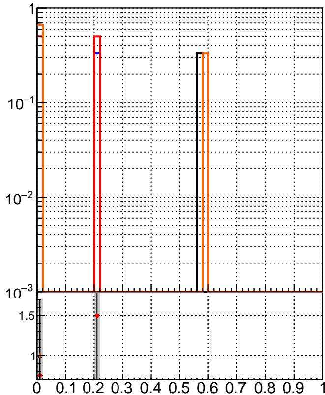
RecoPVAssoc2GenPVNotMatched_missing
