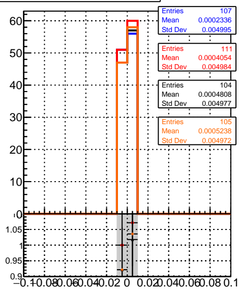
ReconstructedAllAssoc2Gen_X
