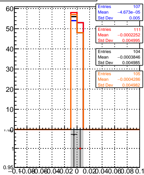
ReconstructedAllAssoc2Gen_Y
