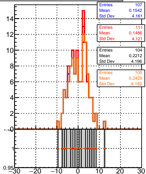
ReconstructedAllAssoc2Gen_NumTracks
