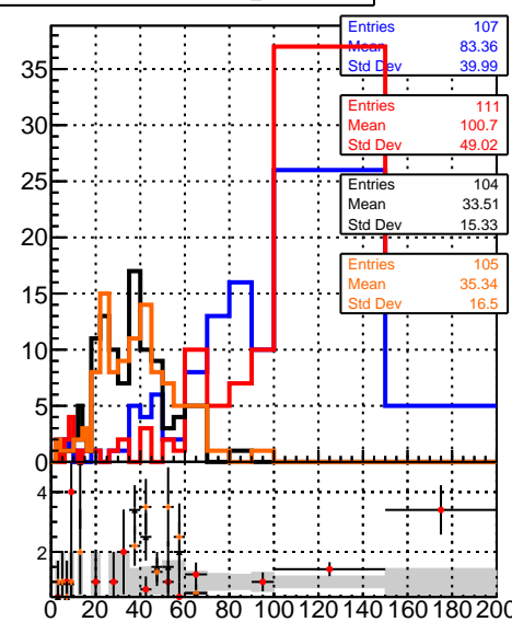
ReconstructedAllAssoc2Gen_NumTracks
