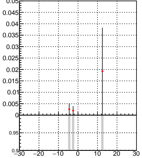
Efficiency vs sim PV z oob
