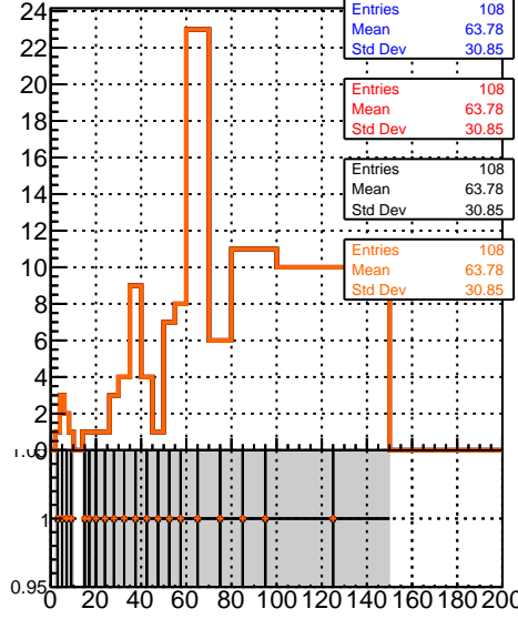
ReconstructedAllAssoc2Gen_NumTracks
