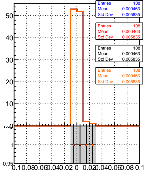
ReconstructedAllAssoc2Gen_Y
