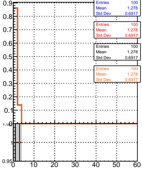
ReconstructedAllAssoc2Gen_NumVertices
