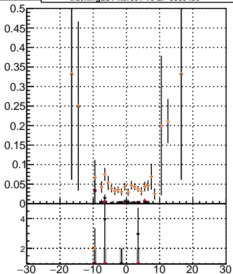
Efficiency vs sim PV z trackingIters01-03fac7e oob trackingLST-Iters01-03fac7e trackingLST-Iters01-T5-2P-33e94a6
