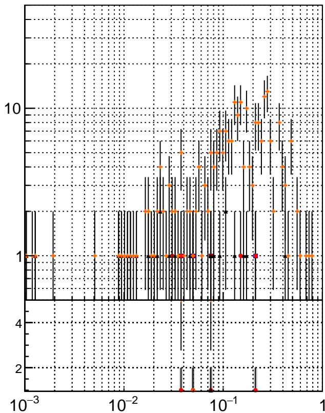
N of associated tracks (simToRec) vs dR
