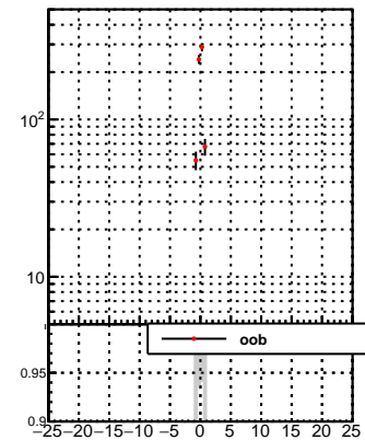
N of reco track vs dx
