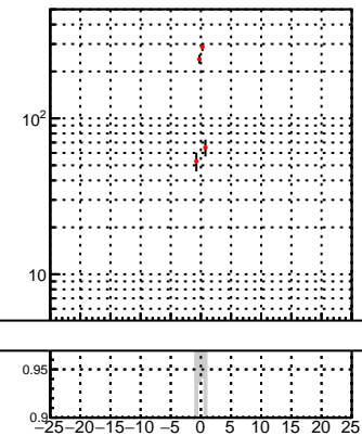
N of associated (recoToSim) tracks vs dx
