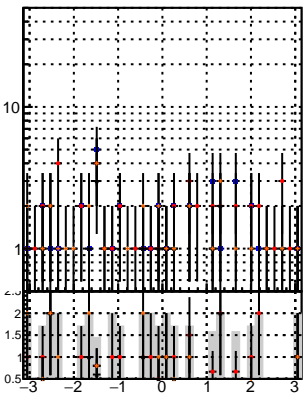
N of reco track vs phi
