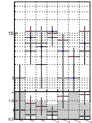
N of reco track vs. \chi^2 trackingIter01-03fac7e trackingLS-Iter01-03fac7e trackingLS-Iter01-15-2P-33e94a6
