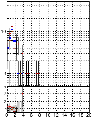
N of reco track vs. \chi^2 trackingIter01-03fac7e trackingLS-Iter01-03fac7e trackingLS-Iter01-15-2P-33e94a6
