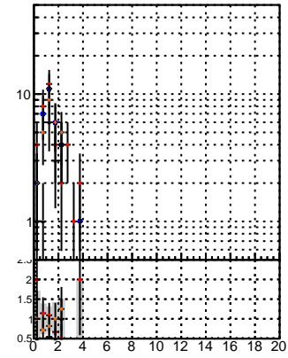
N of reco track vs. \chi^2 trackingIter01-03fac7e trackingLS-Iter01-03fac7e trackingLS-Iter01-15-2P-33e94a6
