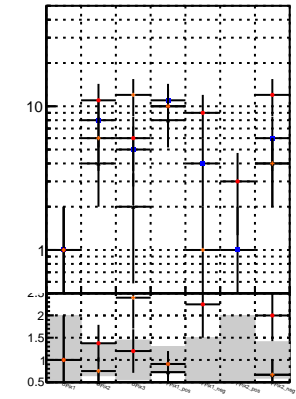
N of reco track vs. \chi^2 trackingIter01-03fac7e trackingIter01-03fac7e trackingIter01-03fac7e
