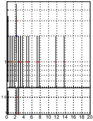
N of reco track vs. \chi^2 trackingIter01-03fac7e trackingIter01-03fac7e trackingIter01-03fac7e
