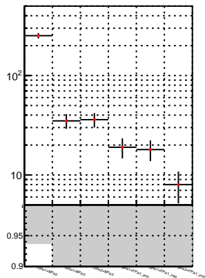
N of reco track vs. \chi^2 oob
