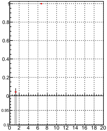
Fake rate vs. —●— oob
