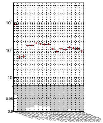
N of reco track vs. \chi^2 oob
