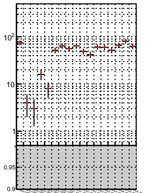
N of reco track vs. \chi^2 oob
