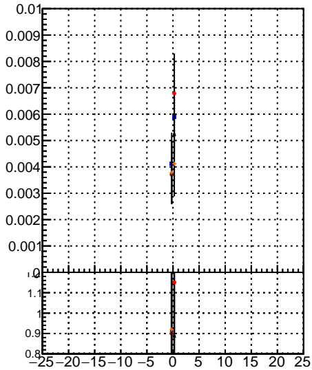
Fake rate vs d trackinglters01-03fac7e blue diamond 800 black square tracking-LT-ltcrs01-03fac7e red triangle tracking-LT-ltcrs01-15-2F-33e94ae orange inverted triangle
