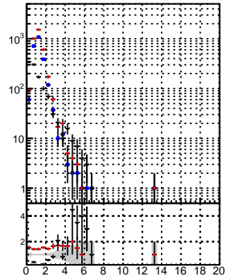
N of associated (recoToSim) tracks vs. \chi^2 —•— trackingiters01-03fac7e —•— 900 —•— trackingLST-iters01-03fac7e
