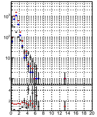
N of reco track vs. \chi^2 —•— trackingiters01-03fac7e —•— 900 —•— trackingLST-iters01-03fac7e
