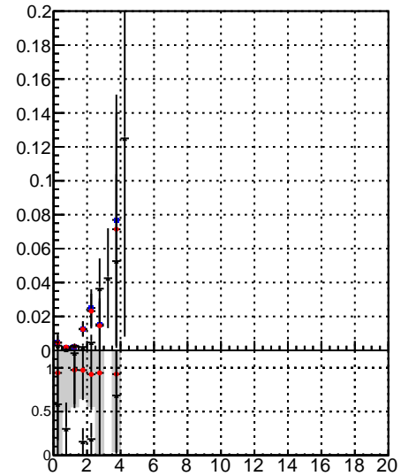
Fake rate vs. trackinglters01-03fac7e good trackingLST-lters01-03fac7e
