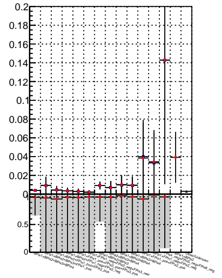
Fake rate vs. trackinglters01-03fac7e good trackingLST-lters01-03fac7e
