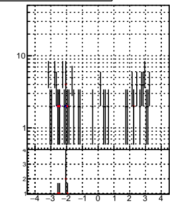
N of associated (recoToSim) duplicate tracks vs d
