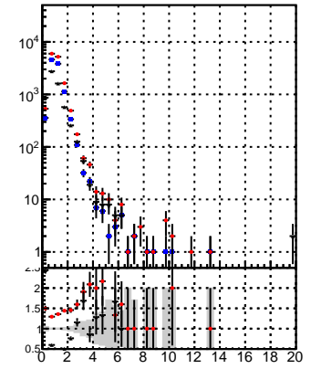
N of reco track vs. \chi^2 ● trackingITers01-03fac7e ● trackingLST-ITers01-03fac7e
