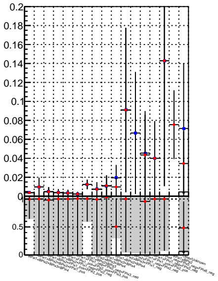
Fake rate vs. trackinglters01-03fac7e 00b trackingLST-lters01-03fac7e
