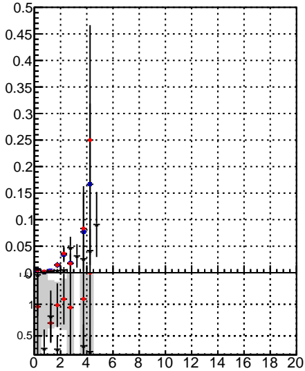
Fake rate vs. trackinglters01-03fac7e 00b trackingLST-lters01-03fac7e
