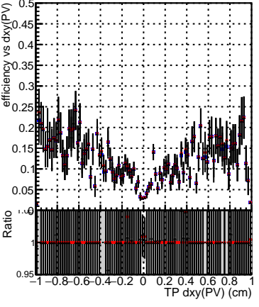
Efficiency vs Dxy(PV) - Legend DQM_ttbarPU_mkFit_Siter DQM_ttbarPU_mkFit_Siter_updatedPR111_update DQM_ttbarPU_mkFit_Siter_updatedPR111_update_fixPropagation
