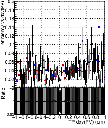
Efficiency vs Dxy(PV) DQM_ttbarPU_mkFit_Siter DQM_ttbarPU_mkFit_Siter_updatedPR111_update DQM_ttbarPU_mkFit_Siter_updatedPR111_update_fixPropagation
