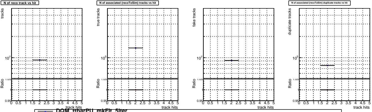
—•— DQM_ttbbarPU_mkFit_5iter —•— DQM_ttbbarPU_mkFit_5iter_updatedPR111_update —•— DQM_ttbbarPU_mkFit_5iter_updatedPR111_update_fixPropagation
