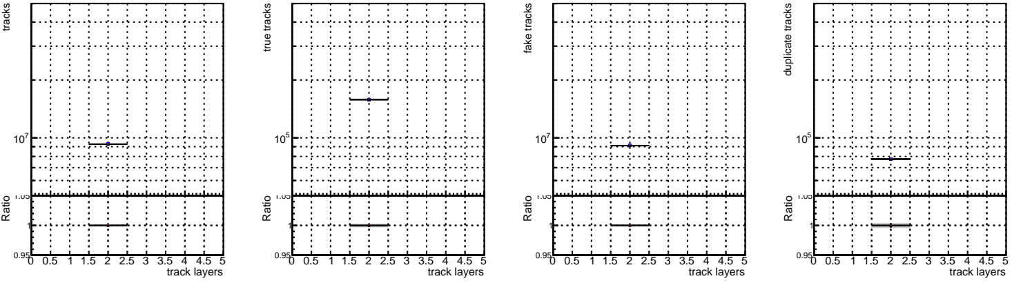
—•— DQM_ttbbarPU_mkFit_5iter —•— DQM_ttbbarPU_mkFit_5iter_updatedPR111_update —•— DQM_ttbbarPU_mkFit_5iter_updatedPR111_update_fixPropagation
