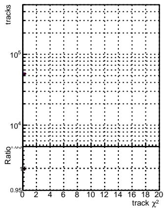
N of reco track vs. \chi^2 for different methods: DGM, tBarPU, mkFit, Siter, updatedPR111, update, fixPropagation
