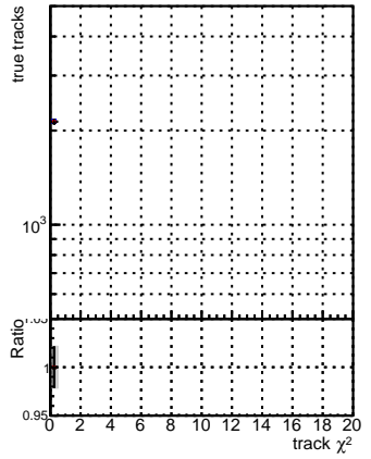
N of reco track vs. \chi^2 for different methods: DGM, ttbarPU, mkFit, Siter, updatedPR111, update, fixPropagation
