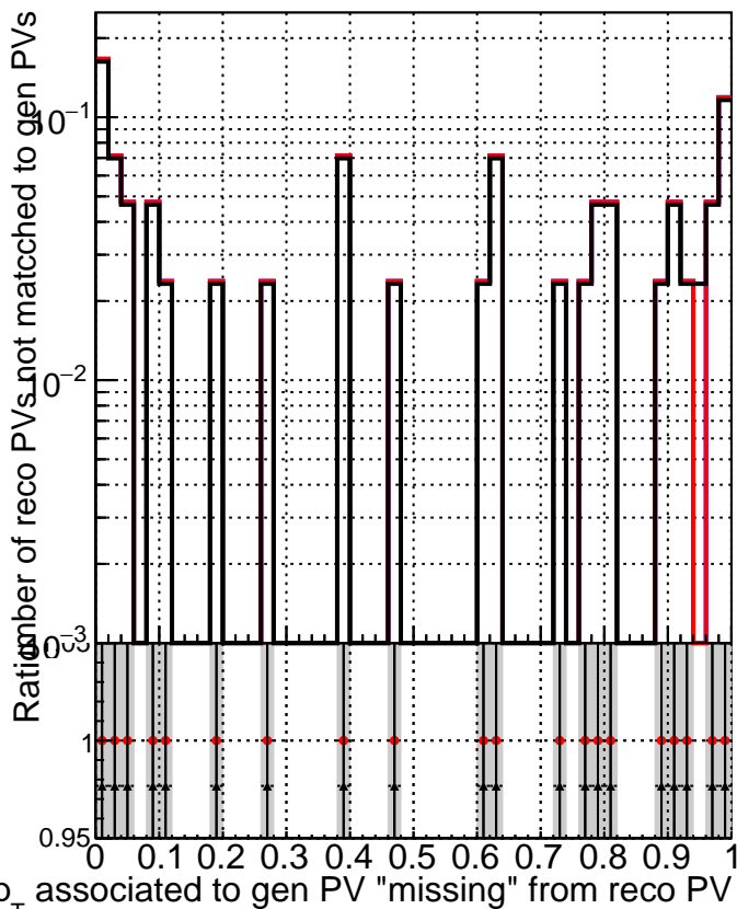
RecoPVAssoc2GenPVNotMatched_missing
