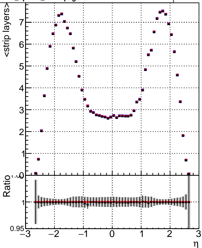
Legend for STRIP hits plots: ■ DQM_ttbarPU_mkFit_5iter ● DQM_ttbarPU_mkFit_5iter_updatedPR111_update ▲ DQM_ttbarPU_mkFit_5iter_updatedPR111_update_fixPropagation
