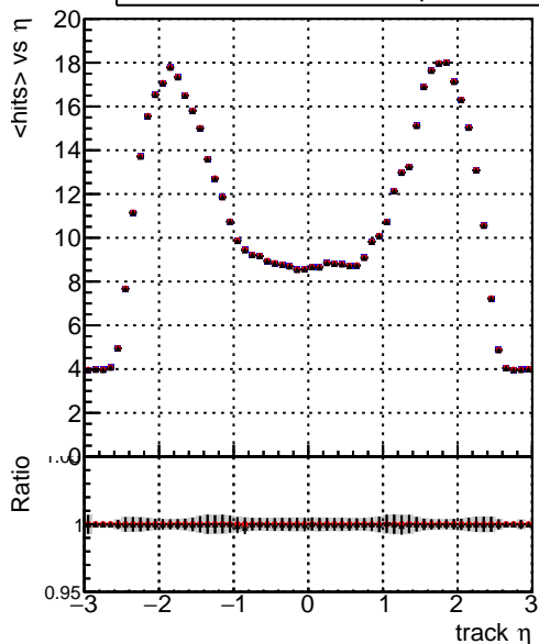
mean hit \eta vs track \eta
