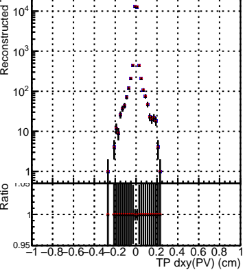
N of associated tracks (simToReco) vs dxy(PV)
