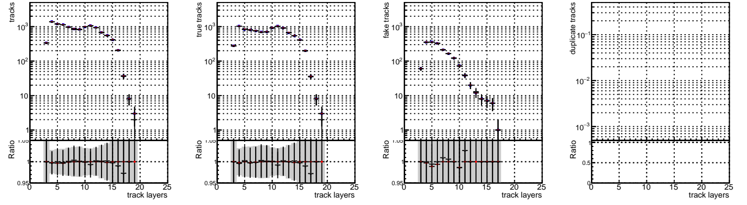
N of reco track vs hit N of associated (recoToSim) tracks vs hit fake tracks N of associated (recoToSim) duplicate tracks vs hit Ratio
