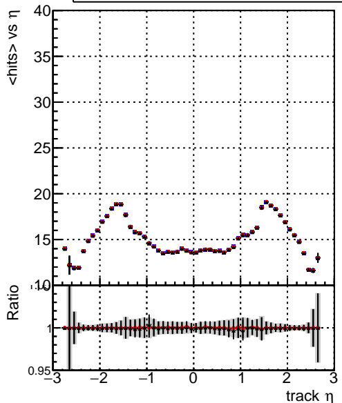
mean hit \eta — DQM_ttbarPU_mkFit_5iter — DQM_ttbarPU_mkFit_5iter_updatedPR111_update — DQM_ttbarPU_mkFit_5iter_updatedPR111_update_fixPropagation
