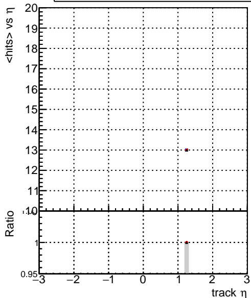
mean hit — DQM_ttbarPU_mkFit_5iter — DQM_ttbarPU_mkFit_5iter_updatedPR111_update — DQM_ttbarPU_mkFit_5iter_updatedPR111_update_fixPropagation
