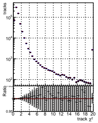
N of reco track vs. \chi^2 ● DGM ● tBarPU ● mFit ● Siter ● updatedPR11 ● update ● fixPropagation
