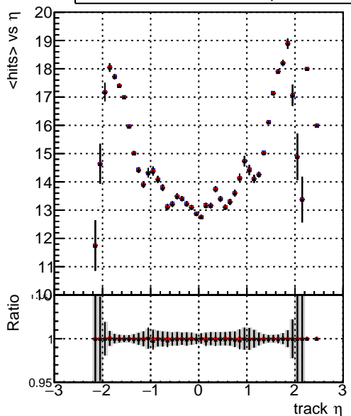
mean hit — DQM_ttbarPU_mkFit_5iter — DQM_ttbarPU_mkFit_5iter_updatedPR111_update — DQM_ttbarPU_mkFit_5iter_updatedPR111_update_fixPropagation
