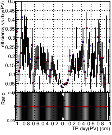
Efficiency —●— DQM_ttbarPU_mkFit_5iter —●— DQM_ttbarPU_mkFit_5iter_updatedPR111_update —●— DQM_ttbarPU_mkFit_5iter_updatedPR111_update_fixPropagation
