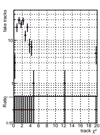
N of reco track vs. \chi^2 for various methods: BGM ttbarPU, BGM ttbarPU, mkFit, Siter, updatedPR11, update, fixPropagation
