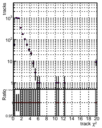
N of reco track vs. \chi^2 for various methods: BGM ttbarPU, BGM ttbarPU, mkFit, Siter, updatedPR11, update, fixPropagation
