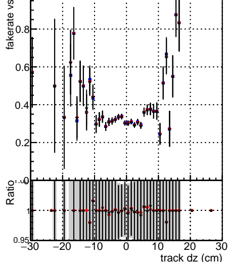
Fake rate vs dx z
