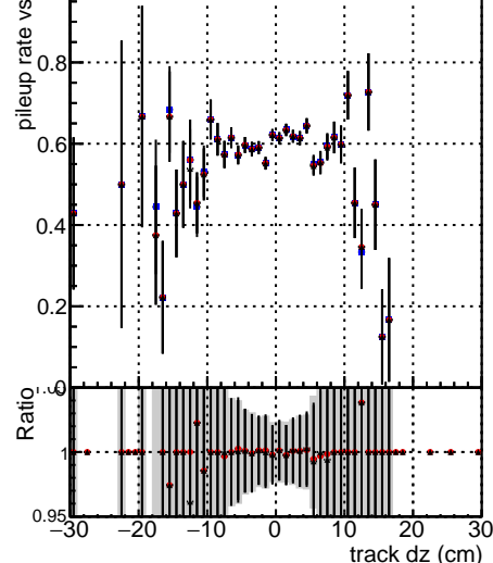
Pileup rate vs dx z
