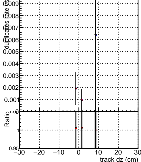
Duplicates Rate vs Dx z
