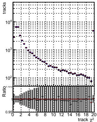
N of reco track vs. \chi^2 for various methods: DGM, ttbar, PU, mkFit, Siter, updatedPR11, update, fixPropagation.
