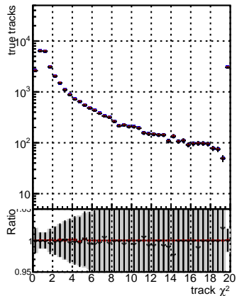
N of reco track vs. \chi^2 for various methods: DGM, ttbar, PU, mkFit, Siter, updatedPR11, update, fixPropagation.
