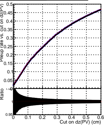
Pileup rate
