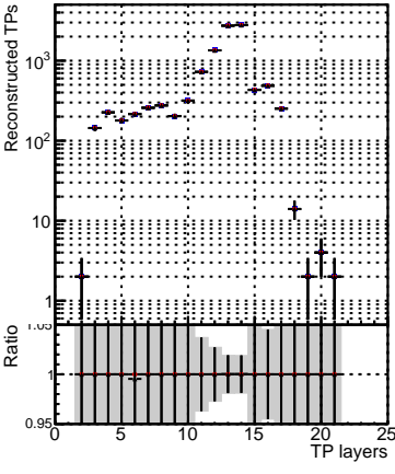
N of sim DQM_ttbarPU_mkFit_5iter DQM_ttbarPU_mkFit_5iter_updatedPR111_update Ratio DQM_ttbarPU_mkFit_5iter_updatedPR111_update_fixPropagation
