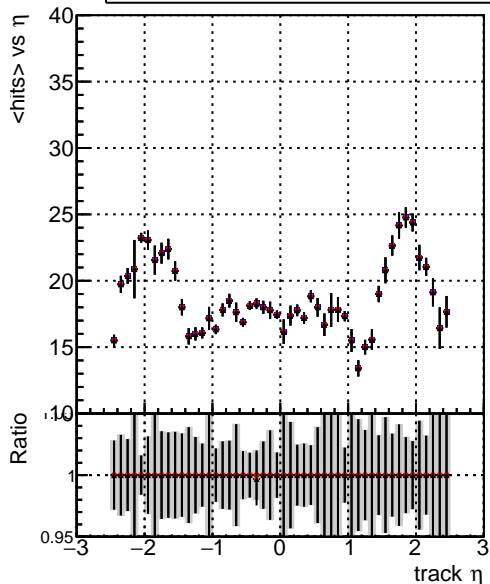
mean hit \eta — DQM_ttbarPU_mkFit_5iter — DQM_ttbarPU_mkFit_5iter_updatedPR111_update — DQM_ttbarPU_mkFit_5iter_updatedPR111_update_fixPropagation
