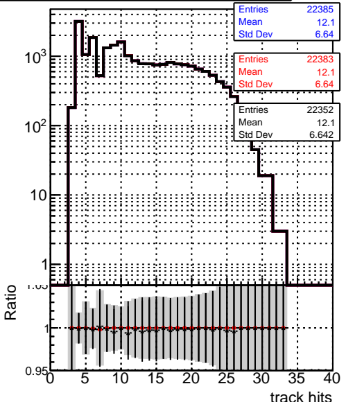
track hits
