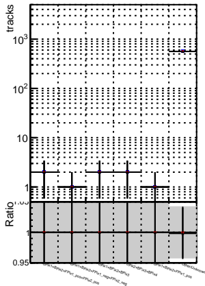
N of reco track vs. ● DGM ● ttbarPU ● mFit ● Siter ● updatedPR111 ● fixPropagation — DGM — ttbarPU — mFit — Siter — updatedPR111 — fixPropagation
