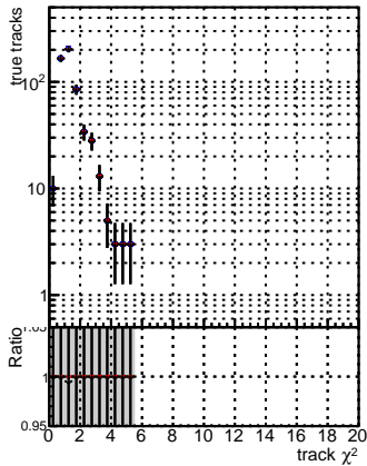
N of reco track vs. ● DGM ● ttbarPU ● mFit ● Siter ● updatedPR111 ● fixPropagation — DGM — ttbarPU — mFit — Siter — updatedPR111 — fixPropagation
