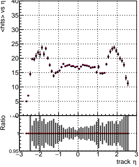
mean hit — DQM_ttbarPU_mkFit_5iter — DQM_ttbarPU_mkFit_5iter_updatedPR111_update — DQM_ttbarPU_mkFit_5iter_updatedPR111_update_fixPropagation
