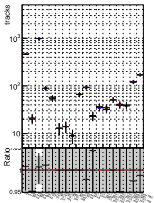
N of reco track vs. \chi^2 —•— DGM —•— tBar —•— PU —•— mkFit —•— Siter —•— updatedPR111 —•— update —•— fixPropagation
