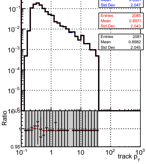
N of reco track vs pT
