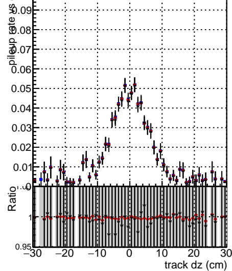
Pileup rate vs dx z
