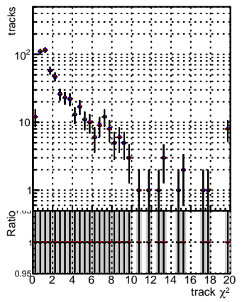
N of reco track vs. \chi^2 for various methods: DGM, tkbar, PU, mkFit, Siter, updated, PR111, update, fix, Propagation
