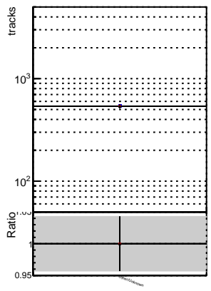
N of reco track vs. \chi^2 for various methods: DGM, tkbar, PU, mkFit, Siter, updated, PR111, update, fix, Propagation
