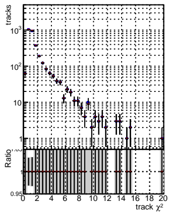
N of reco track vs. \chi^2 for various methods: DGM (black), ttbar (red), PU (green), mkFit (blue), Siter (purple), updatedPR111 (orange), update fixPropagation (grey).
